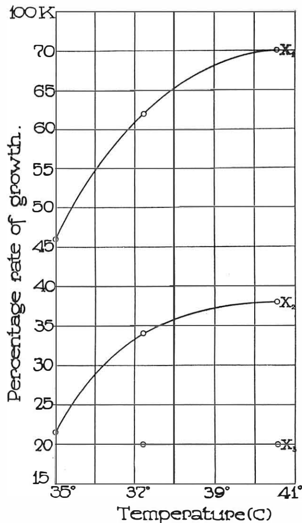
FIG. 2.—The relation between temperature and the relative-rate of growth, \lambda , for phases X 1 , X 2 , and X 3 . (cf. Fig. 1).
