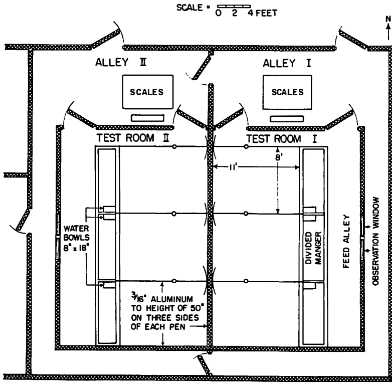
Figure 1—Floor plan of testing areas within the Psychroenergetic Laboratory. Test Room I and Alley I were maintained at 50° F and Test Room II and Alley II at 80° F. The calves were weighed on the alley scales but otherwise remained in the test rooms throughout the tests.
