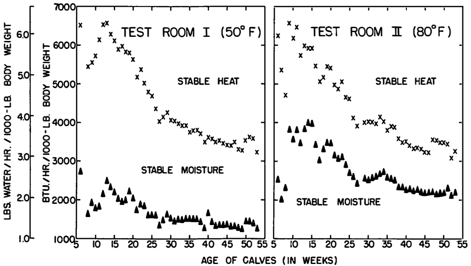
Figure 2—The stable heat (total) and stable moisture (latent heat) dissipated within the 50° and 80° F test rooms. Each datum point represents the weekly average, using the results from daily ventilation exchange calculations (Table 2). These records were obtained with 9 calves in each test room, three each of Jersey, Brown Swiss, and Holstein. Stable moisture may be read on either the heat or the water scale. A value of 1044 Btu/lb. of moisture was used to equate moisture and heat.
