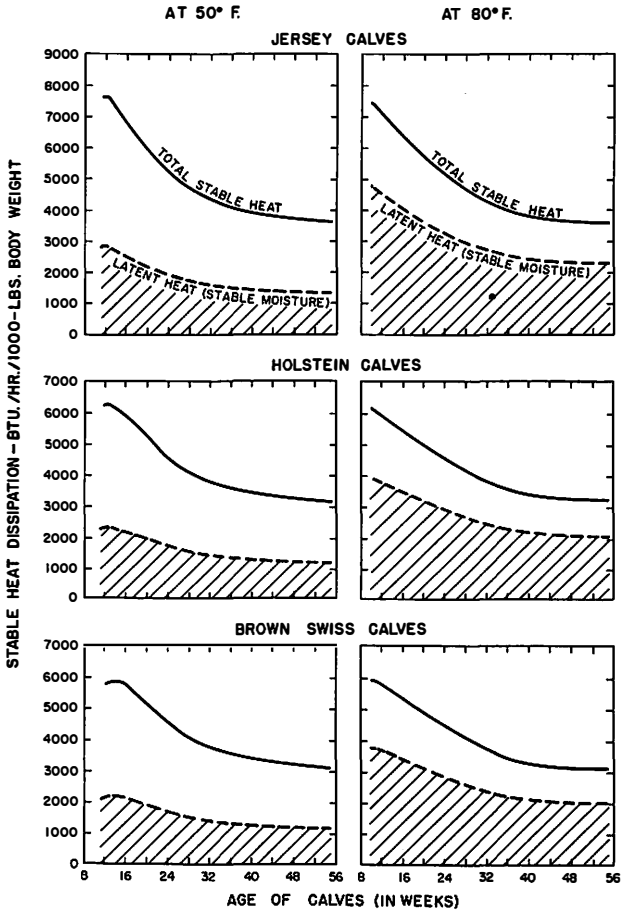
Figure 3—Predicted stable total heat and stable latent heat (stable moisture) dissipation at 50° and 80° F for three breeds of dairy calves and with pens cleaned daily. Total stable heat curves are from test room (3 breeds) ventilation exchange measurements—scaled upward or downward according to breed differences in animal heat production. 2 The ratios of latent to total stable heat (from room ventilation exchange measurements) were applied to the predicted total stable heat curves to obtain the predicted stable moisture curves.
