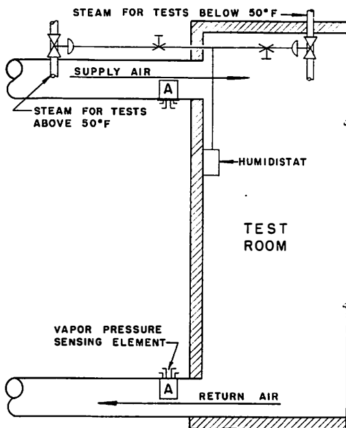
Fig. 1. Methods Used to Measure and Control Humidity.
