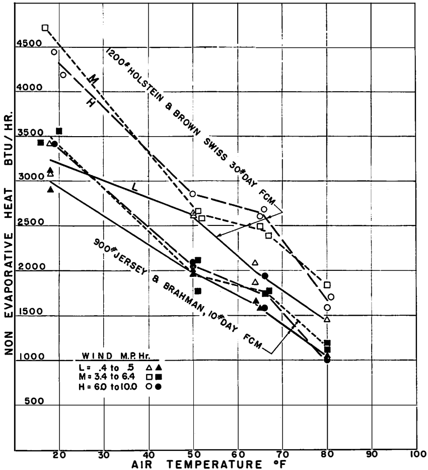
Fig. 13. The Effect of Wind on Non-evaporative Heat Loads at Various Temperatures, 1951-52 Data. These data were derived by subtracting adjusted latent heat (1054 Btu per pound total test room vapor) from adjusted total heat. At constant wind, sensible heat is directly proportional to differences between animal body temperature (near 100° F) and air temperatures.
