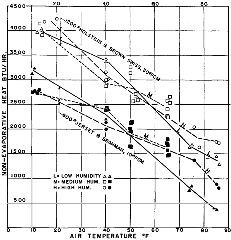
Fig. 6. The Effect of Humidity on Adjusted Non-evaporative Heat Loads at Various Temperatures, 1950-51 Data. All values were adjusted to the approximate mean body weight and milk production of their respective test groups. Evidently increases in total heat load due to high humidity at 85° F may be attributed to non-evaporative sources. Note the uniform range of measurements for both groups at all temperatures. The heat of vaporization was assumed to be 1054 Btu per pound.
