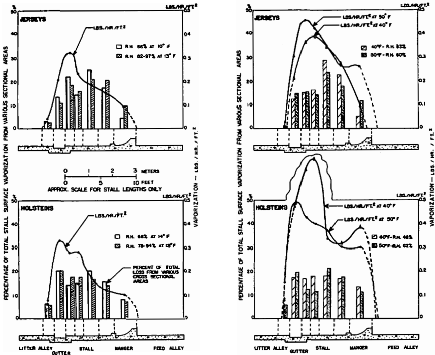
Fig. 7. Percent of Test Room Surface Evaporation From Various Segments of the Stall. See references (2) and (3).
