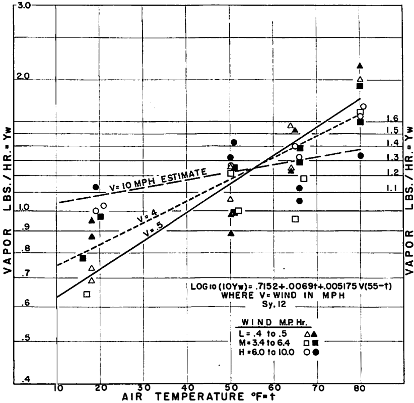
Fig. 12. The Effect of Wind on Total Test Room Vaporization at Various Temperatures, 1951-52 Data. Data are the same as in Figure 11 except that adjustments were made to a 1000-pound body weight base and a 20-pound FCM base. Solid points represent Jersey and Brahman cows, open points represent Holstein and Brown Swiss cows. The crossing point of the curves at 55° F was arbitrarily selected after inspection of Figure 11. Wind apparently affects the sum of animal and stall vaporization at 20° and 80° F. The differences between the ½ and 10 mph curves are about equal but opposite in sign at 20° and 75° F.
