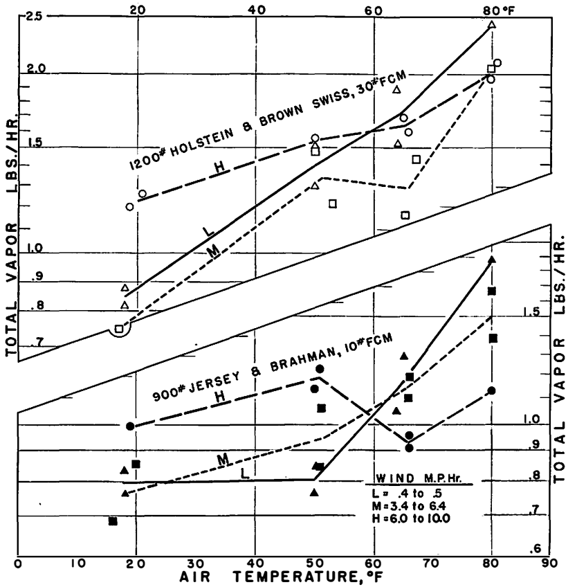
Fig. 11. The Effect of Wind on Adjusted Total Test Room Vaporization at Various Temperatures, 1951-52. All values were adjusted to an approximate mean body weight and milk production for their respective test groups as per method described in Figure 4. The respective base points for each group are shown in the Figure. Wind increased the total test room vaporization within a 16-21° F temperature range and decreased total test room vaporization at 80° F. The effect of wind probably reaches a minimum somewhere between 50° and 65° F.
