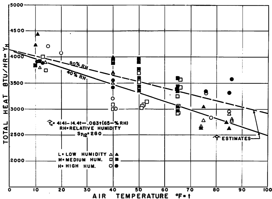
Fig. 3. Estimated Effects of Humidity on Total Heat Load at Various Temperatures, 1950-51 Data. All values were adjusted to common body weight and milk production bases as described in Figure 2. However, since both groups are together the bases of 1000-pound body weight and 20 pounds FCM were used. Solid points represent Jersey and Brahman cows. The open points represent Brown Swiss and Holstein cows. Although the multiple correlation coefficient of 0.78 for 60 degrees of freedom is significant, the humidity coefficient is significant at only the 5 percent level. Note the wide range of data at 40° and 50° F. Time effects for the intermittent periods of 50° F do not seem to be consistent (see Tables 1 and 2).
