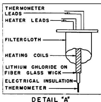
Fig. 1. Methods Used to Measure and Control Humidity.
