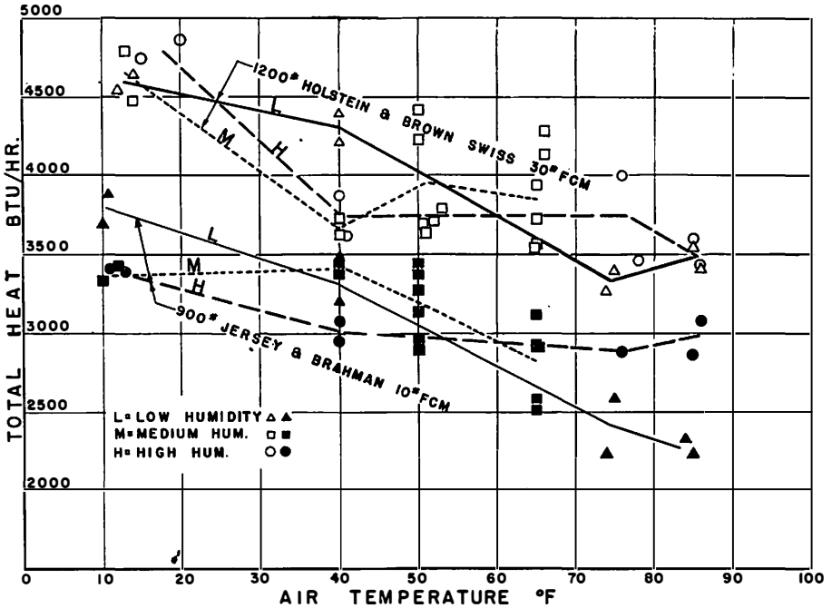
Fig. 2. Effect of Humidity on Total Heat Load at Various Temperatures, 1950-51 Data. All values were adjusted to common body weight and milk production bases near the average weight and production level of each of the two test groups. The base values are shown with the curves for their respective groups. Milk production adjustments were made at 20 Btu/hr. per pound of 4 percent FCM/day above or below respective base points. Weight adjustments were made according to the 0.75 power of the ratio of base weight to actual weight. For example, the first total heat load value of Table 1 was adjusted as follows: [3770 - 20(28-10)] [900/902]^{0.75} = 3400 \text{ Btu/hr.}
