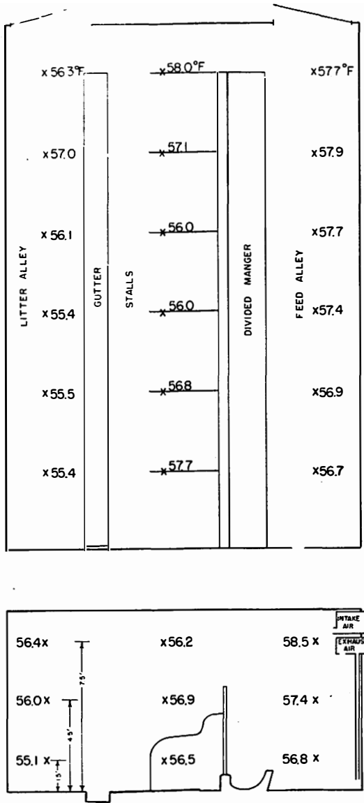
Fig. 3—An example of the air temperature variation within the test room during the mean temperature period of the 40 to 70° F diurnal temperature cycle. The values in the upper section are those measured 4.5 ft. above the floor. Those in the lower section represent average values for the six stalls. The stalls are numbered beginning with 1 at the top of the page. The exhaust air temperature during these measurements increased from 55.3° to 57.1° F. Intake temperatures ranged from 50.6° to 54.9° F.
