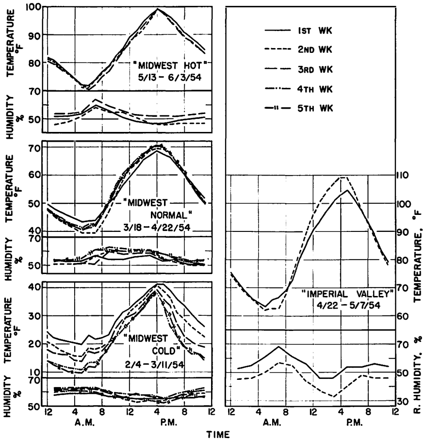
Fig. 2.—The schedule of temperature and relative humidity for each week of the spring, 1954, tests. Each diurnal curve was plotted from average temperatures of one-hour periods.
