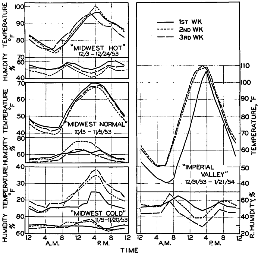
Fig. 1—The schedule of temperature and relative humidity for each week of the fall, 1953, tests. Each diurnal curve was plotted from average temperatures of one-hour periods.
