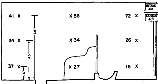
Fig. 4—Air velocities within the test room during the diurnal temperature cycles. The upper section shows the velocities at each position indicated by an "X". The three values of a set are given according to height above the floor, the upper one representing a height of 7.5 ft., the next 4.5 ft., and the lowest 1.5 ft. The lower section of the figure shows average values for the six stalls. The velocity around the cows averaged about 30 feet per minute.
