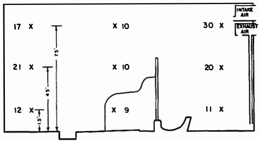
Fig. 5—Light intensities (in foot candles) in the test room during the diurnal temperature cycle. The measuring stations are designated by an "X". There was sufficient light near the floor to read the fine graduations on instruments.
