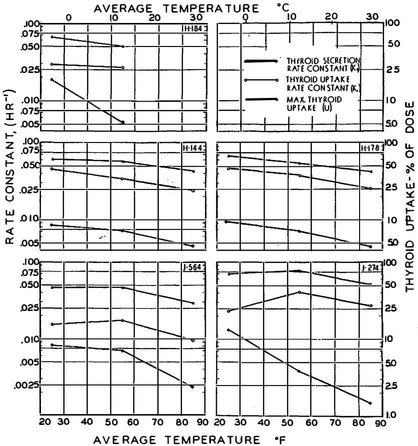
Fig. 3. — Thyroid activity of Jersey and Holstein cows. Semi-logarithmic plots of the rate constants for thyroid uptake, k_1 , and hormone release, k_2 , and the maximum uptake of I^{131} by the thyroid gland, U , as a function of the average temperature. Note decreasing trend of parameters with increasing average temperature.
