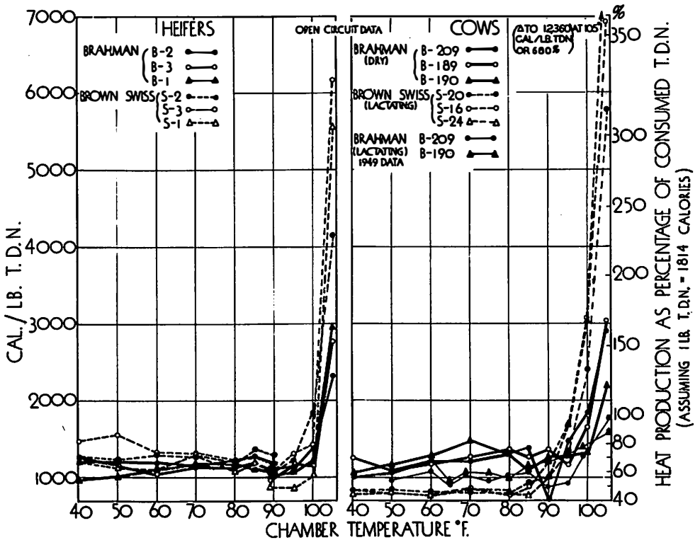
Fig. 3.—Ratio of heat production to total digestible nutrient consumption in Brahman and Brown Swiss heifers (left) and dry Brahman and lactating Brown Swiss cows (right) in relation to increasing temperature. The left-hand scale expressed in calories per pound TDN and the right-hand scale expressed in heat production calories as a percentage of consumed TDN calories (1 lb. TDN = 1814 calories) apply to both the heifer and cow data.
