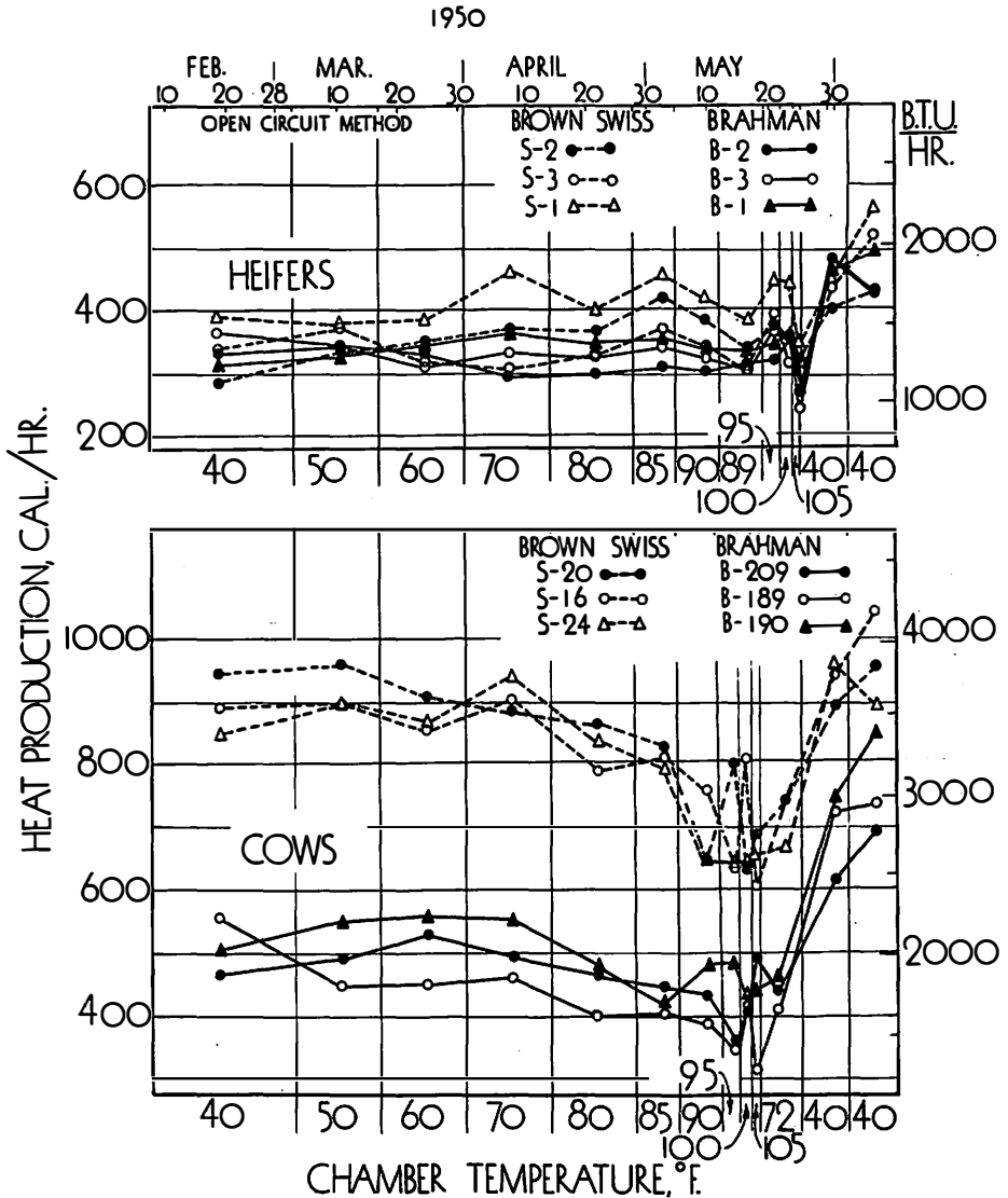
Fig. 1.—Comparison of the heat production of individual Brown Swiss and Brahman heifers (top) and lactating Brown Swiss and dry Brahman cows (bottom) in relation to gradually increasing environmental temperature.
