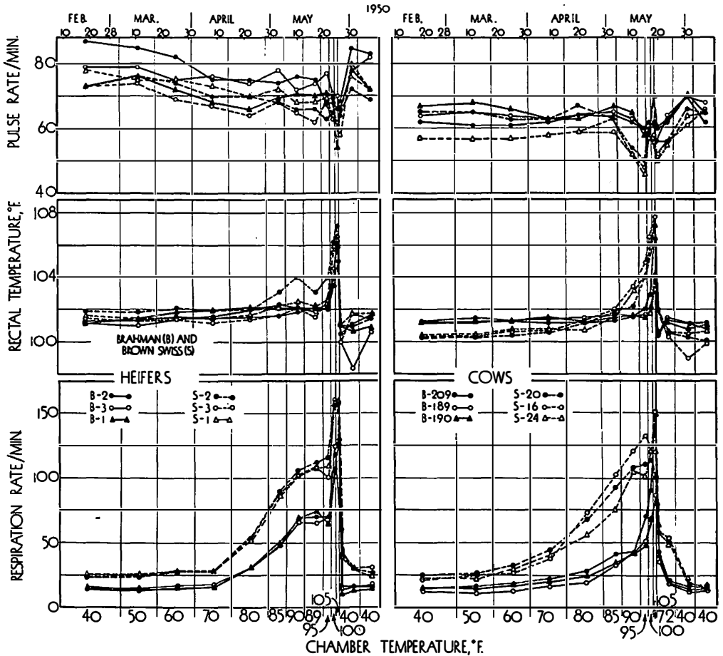
Fig. 4.—Pulse rate, rectal temperature, and respiration rate in Brown Swiss and Brahman heifers (left) and in lactating Brown Swiss and dry Brahman cows (right) in relation to gradually increasing environmental temperature.
