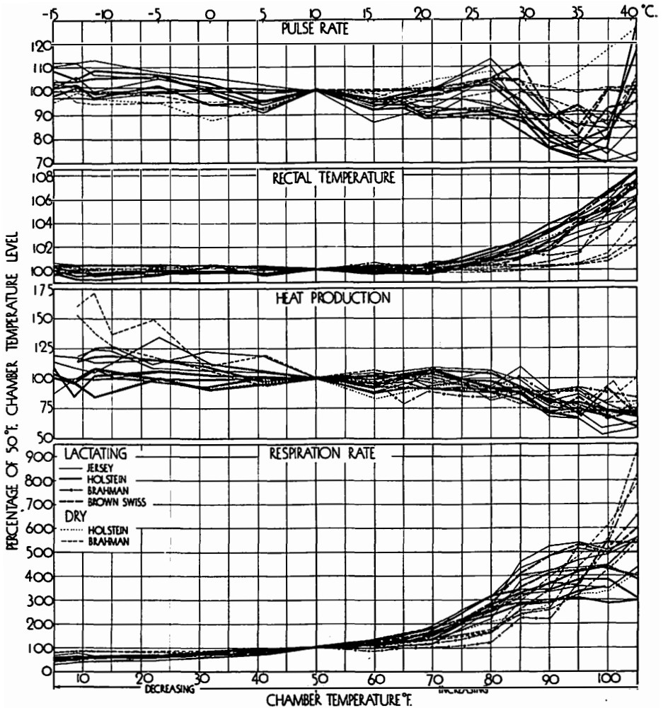
Fig. 5.—Summary of present and previously reported heat production and cardiorespiratory data on individual Jersey, Holstein, Brahman, and Brown Swiss cows for environmental temperatures 5° to 105°F, expressed as percentages of the respective levels at 50°F environmental temperature.
