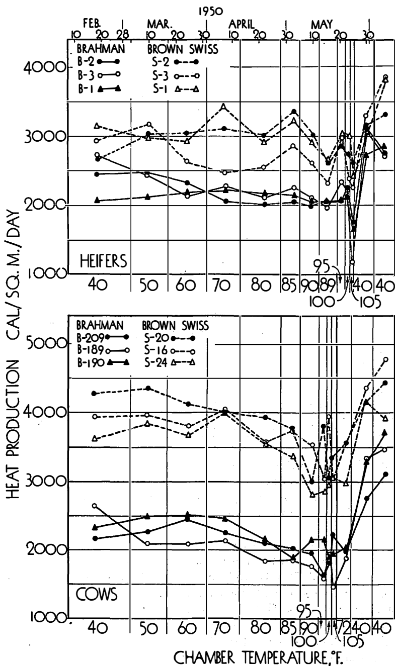
Fig. 2.—Heat production per square meter of surface area in individual Brown Swiss and Brahman heifers (top) and lactating Brown Swiss and dry Brahman cows (bottom) in relation to gradually increasing environmental temperature.
